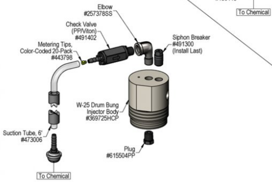
CONFIGURATION #2 Plug on Bottom, Chemical Suction on Top
