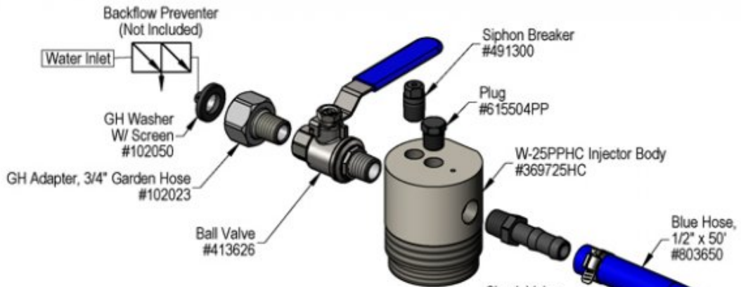
CONFIGURATION #1 Plug on Top, Chemical Suction on Bottom
